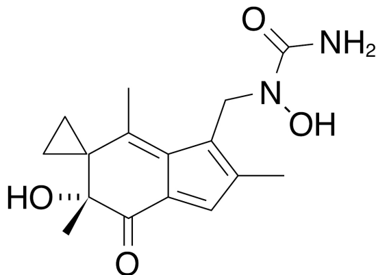
LP-184 Chemical Structure
