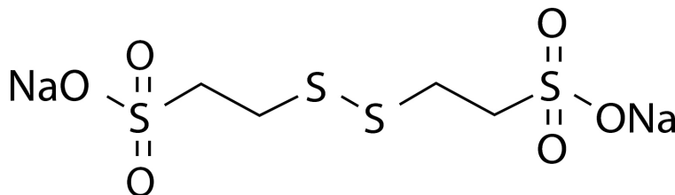
LP-300 Chemical Structure
